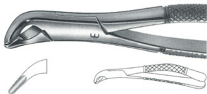
Cryer for Lower Incisors, Cuspids, and Bicuspids WI-021-076 # 151 A
